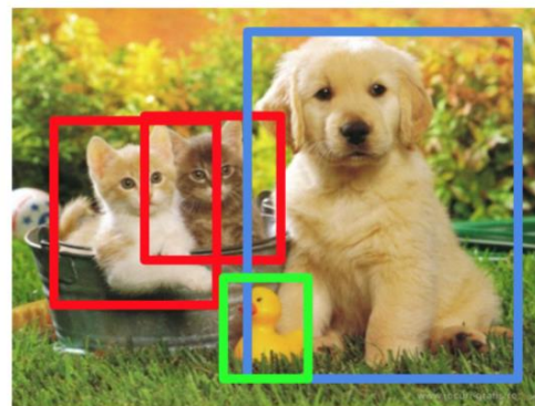
Object Detection
